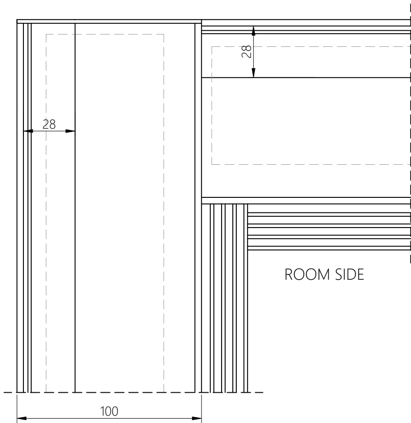
PLAN VIEW
