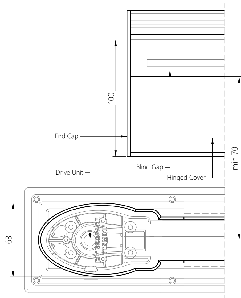
MOTOR BOX TTSMB1F & HEAD BOX S100x100NS
