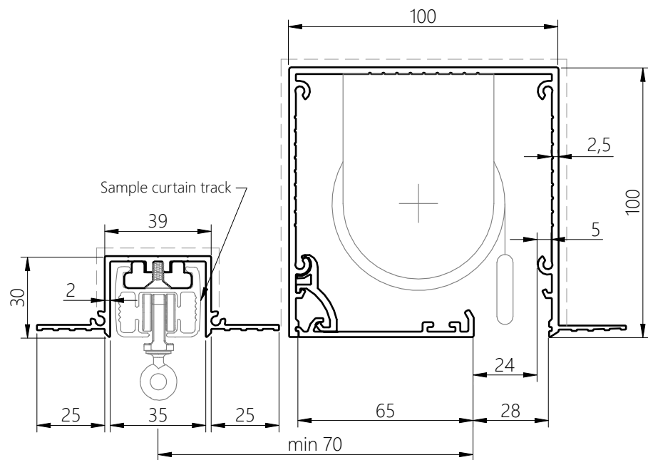
TRACK PROFILE TT1F & HEAD BOX S100x100NS
