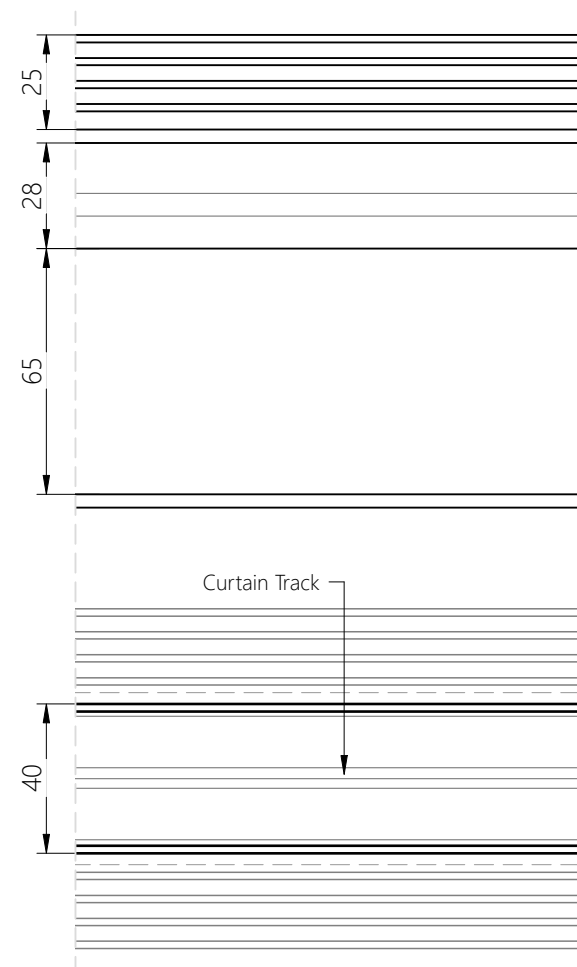
TRACK PROFILE TT1F/TT2F & HEAD BOX
